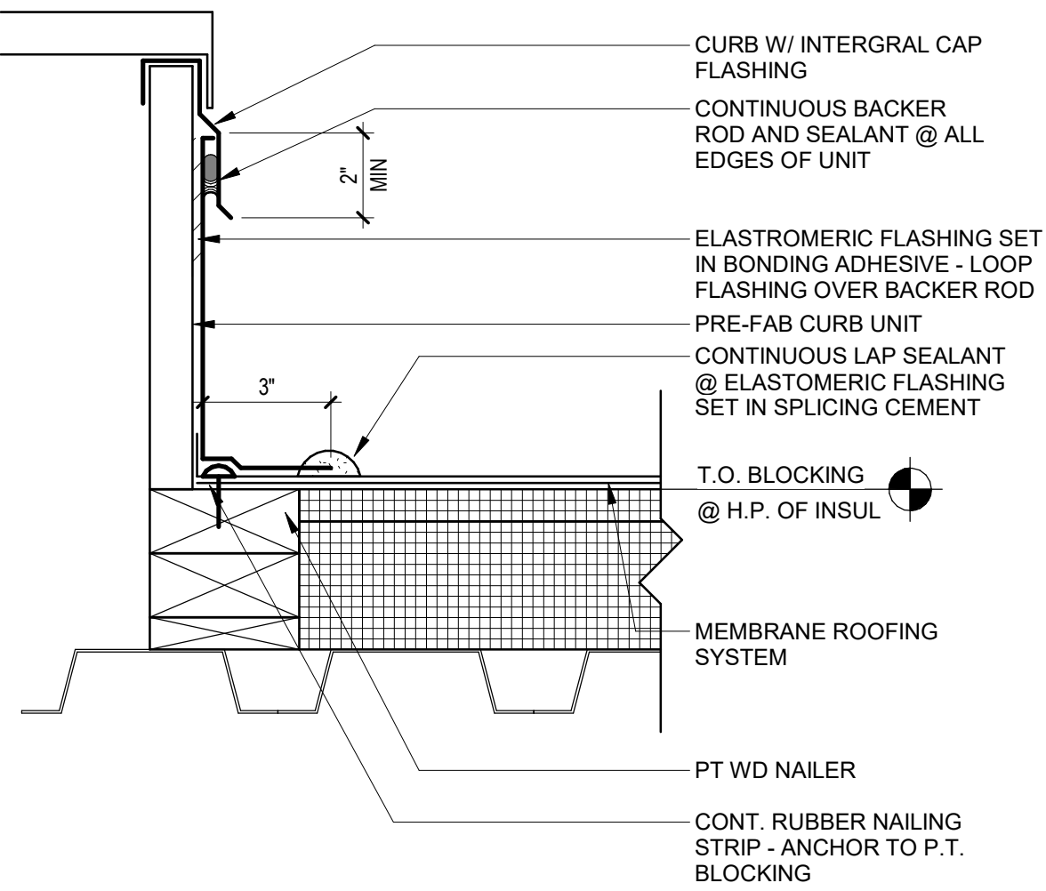
VERTICAL TERMINATION @ ROOF TOP AHU
