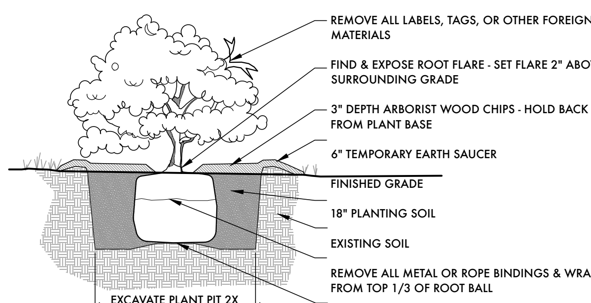
3 SHRUB PLANTING DETAIL
